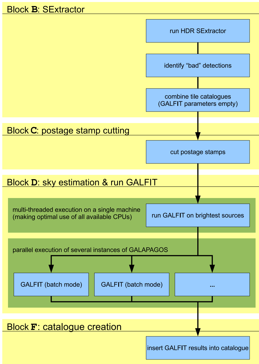
Figure 1. Code structure. A yellow background indicates the four main blocks, labelled according to the nomenclature of the GALAPAGOS setup file (see Fig. A1). Fitting objects with GALFIT (Block (D)) is a two-stage process (see Sec. 3.5), which typically requires more than 90% of the total computation time (green background). We mark smaller tasks by blue boxes. For further details see Sec. 2.
