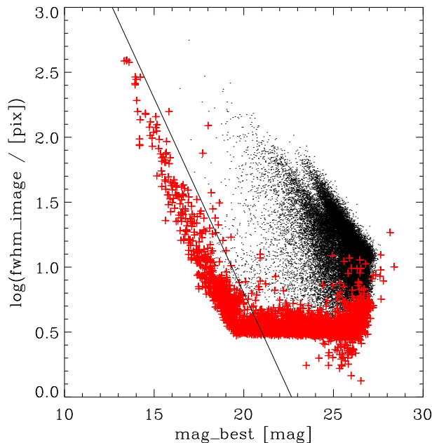
Figure 13. Treatment of saturated stars. Here we show source detections from the STAGES survey in the \log(\text{fwhm\_image}) vs. \text{mag\_best} plane. Red pluses mark objects identified as stars (see Gray et al. 2008). The line indicates the cut used to identify saturated stars (left of the line). Black dots show other (extragalactic) sources.
