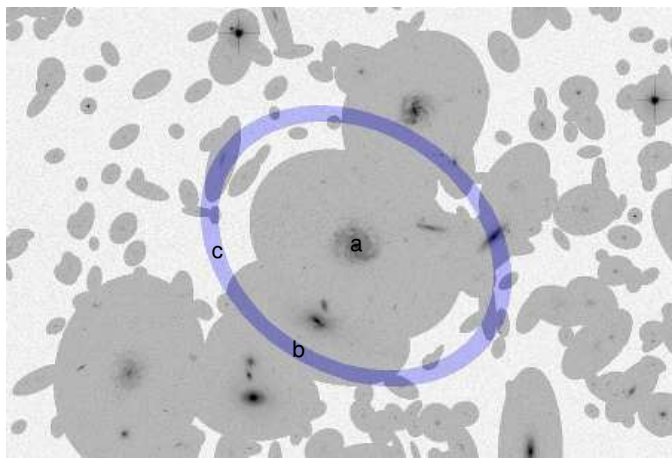
Figure 5. Sky estimation. Left: The average flux f measured in elliptical annuli (blue) centred on an object (here a ) determines the background level. In each annulus, we exclude regions surrounding other sources from the calculation (shaded area). For the indicated annulus, we exclude dark blue shaded regions b – only light blue regions c define the average background flux. Right: Flux f measured in an elliptical annulus as a function of radius r . a : Starting radius. b : Slope (indicated by the diagonal lines) turns positive for the first time, e.g. due to galactic structure at large radii. c : Slope turns positive for the second time. Here we stop the iteration. d : We compute slope measurements from the last n sky estimates (here: n=5 ; n is a user parameter). e : The adopted background sky level. See Sec. 3.4 for details.
