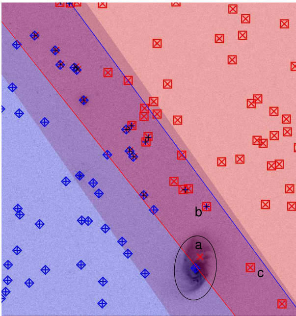
Figure 4. Combining SETRACTOR catalogues from neighbouring tiles. The left image (blue area) extends out to the right (blue) diagonal line; the right image (red area) extends out to the left (red) line. Shaded areas outside of the lines corresponding to the respective image did not receive sky flux. Pluses (blue) indicate source detections (hot and cold already combined) from the left (blue) image; crosses (red) mark detections from the right (red) image. Diamonds (blue) highlight objects that are contained in the combined catalogue if they originated from the left (blue) image; boxes (red) highlight those that were taken from the right (red) image. Catalogue combination is based on the SETRACTOR ellipses (see Sec. 3.2). Such an ellipse is shown in case a). The source from the right image (red) is rejected as it lies inside an ellipse of a detection in the left image (blue), which is further away from the respective image boundary (blue and red lines). For the same reason in case b) the red source is kept. The detection in case c) does not even have a counterpart in the other catalogue.
