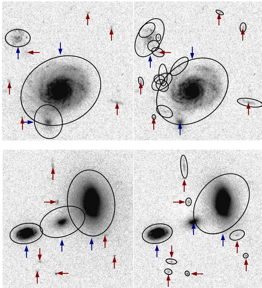
Figure 2. Combining “hot” and “cold” SExtractor catalogues. The two panels ( upper and lower ) show examples of a cold (left side) and a hot (right side) SExtractor extraction. Ellipses indicate the SExtractor Kron ellipses of the detected sources. Arrows mark objects from the hot (red) and the cold (blue) catalogue that were incorporated into the combined catalogue. Additional hot sources not marked with arrows (e.g. in the upper right panel) were excluded from the combined catalogue as described in detail in Sec. 3.1.
